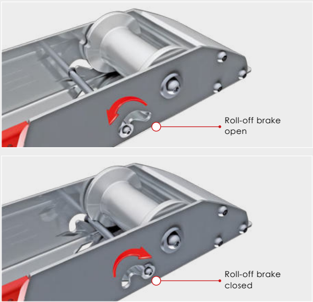
Roll-off brake function
