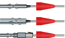
Application cable pulling loop
